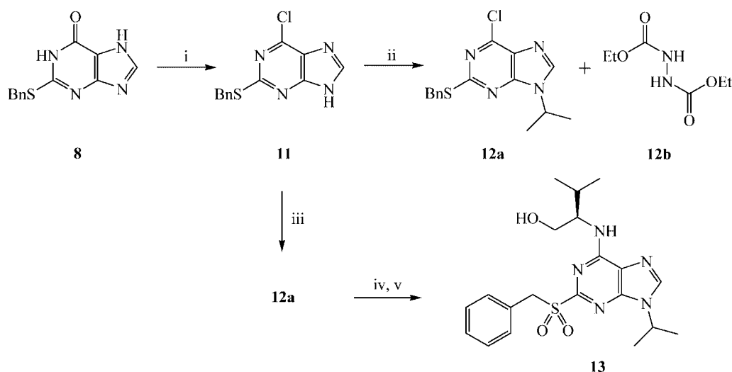
Scheme 5. Conditions: i) \text{POCl}_3 , DMA, \text{NEt}_4\text{Cl} , MeCN, 120^\circ\text{C} (89%) ii) \text{Ph}_3\text{P} , i\text{PrOH} , THF, -10^\circ\text{C} then DEAD, -10^\circ\text{C} to room temp. (20%) iii) \text{Ph}_3\text{P} , DIAD, THF, -50^\circ\text{C} then i\text{PrOH} , -50^\circ\text{C} to room temp. (69%), iv) \text{MgSO}_4 , m\text{-CPBA} , DCM (100%) v) D-valinol, THF, \Delta
